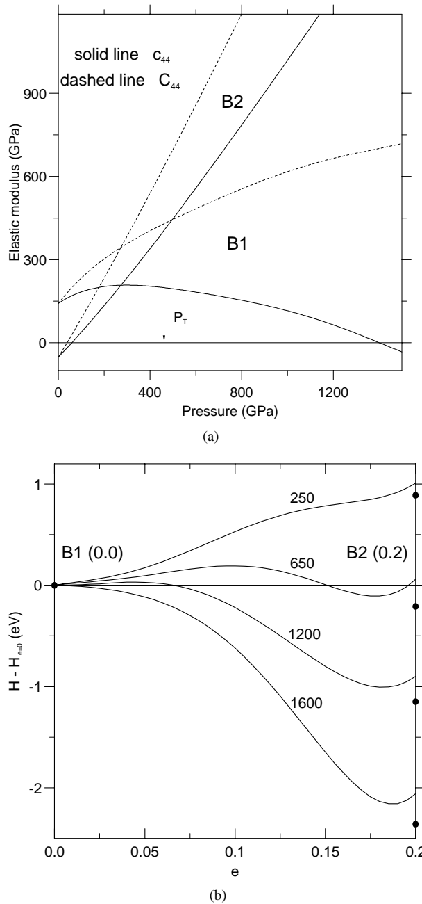
Figure 1. (a) The pressure variation of c_{44} and C_{44} for the B1 and B2 phases of MgO. The arrow indicates the B1–B2 transition pressure ( P_T ) predicted by thermodynamic equality of enthalpies. (b) The relative enthalpy of the deformed B1 structure of MgO versus the shear strain ( e ) at different pressures (indicated by numbers, in GPa). The solid circles represent the relative enthalpies of the optimized structures. Note that at e = 0.2 , the strained B1 lattice has undergone a volume contraction of 10%, and thus represents B2 at a higher pressure.
