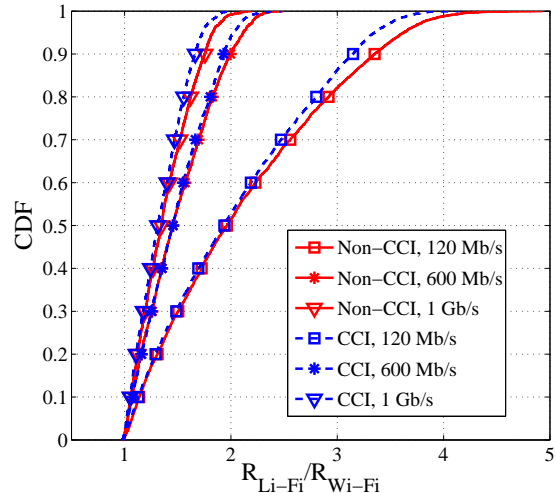
Fig. 9. CDF of the user data ratio R_{Li-Fi}/R_{Wi-Fi} in non-CCI and optical CCI case. The user density is set to be 0.2 person/m 2 , which is normal in the indoor office scenario. ( \eta = 1 )
