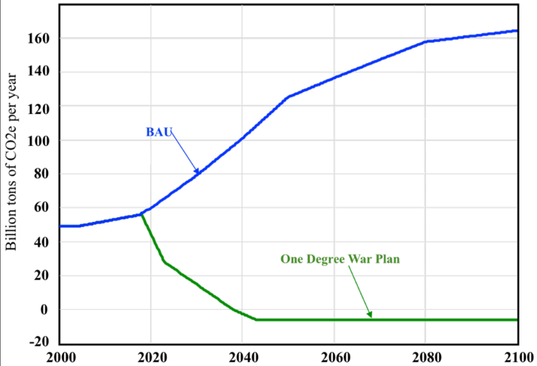
Figure 1 GHG Emissions into the Atmosphere – GtCO 2 e/year
