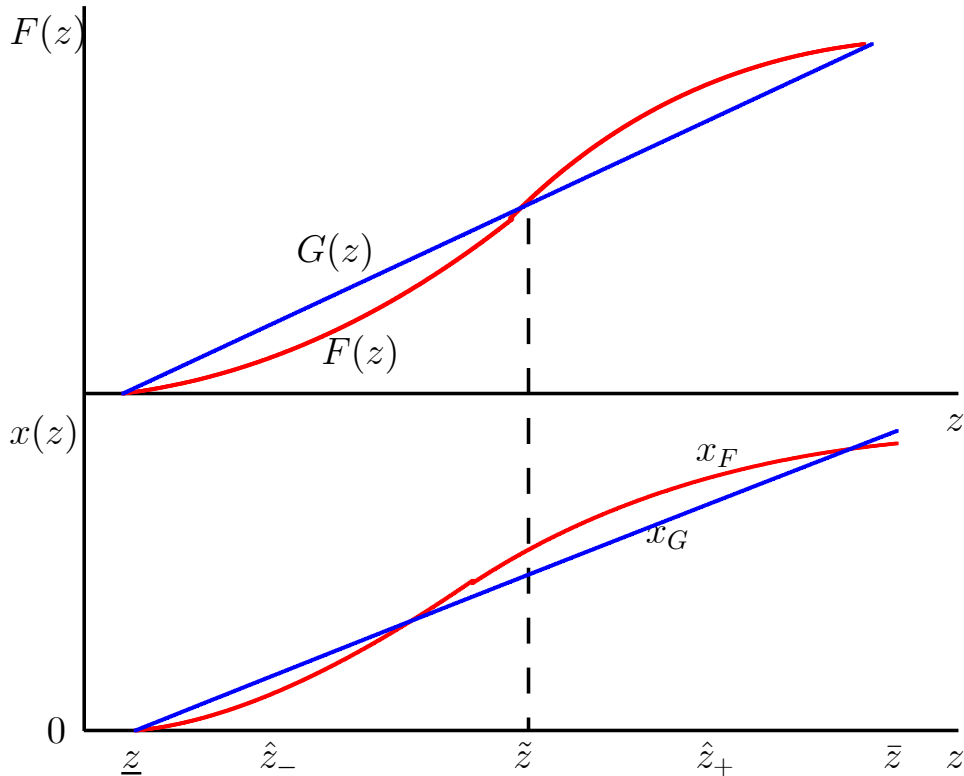
Figure 3: Comparative Statics for an All Pay Auction.
