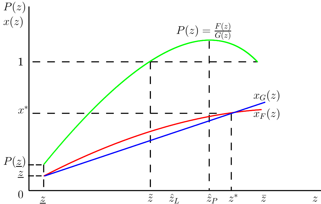
Figure 2: Comparative Statics for a First Price Auction
